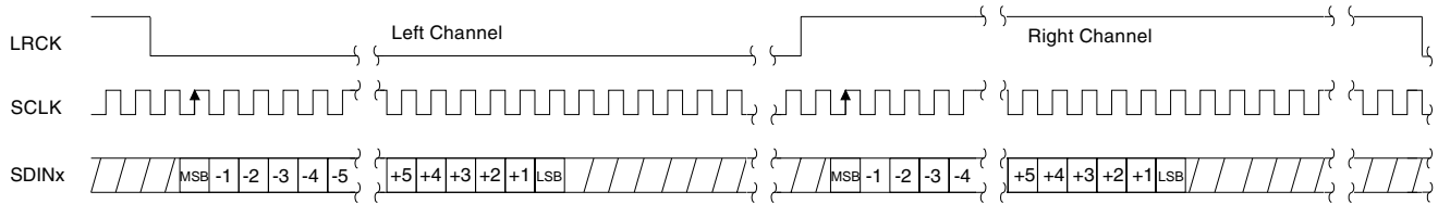
Figure 34. Format 1 - I 2 S up to 24-bit Data
